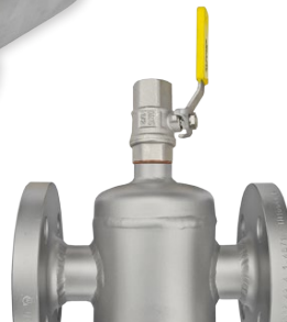
Type PSA DN100 with flange connection
