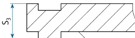
Nut-Feder Form CD groove-tongue Form CC
